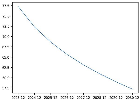
Figure 1.9: Futures curve for the December CL contract
