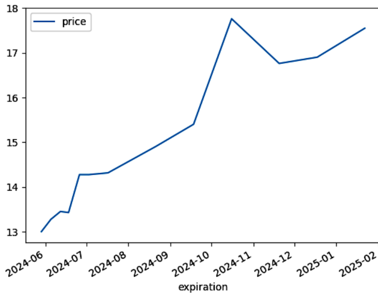
Figure 1.7: VIX futures curve
