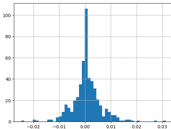
Figure 8.4: Histogram of daily portfolio returns
