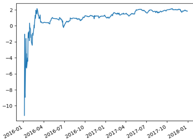
Figure 8.5: Plot of the rolling Sharpe ratio of the algorithm
