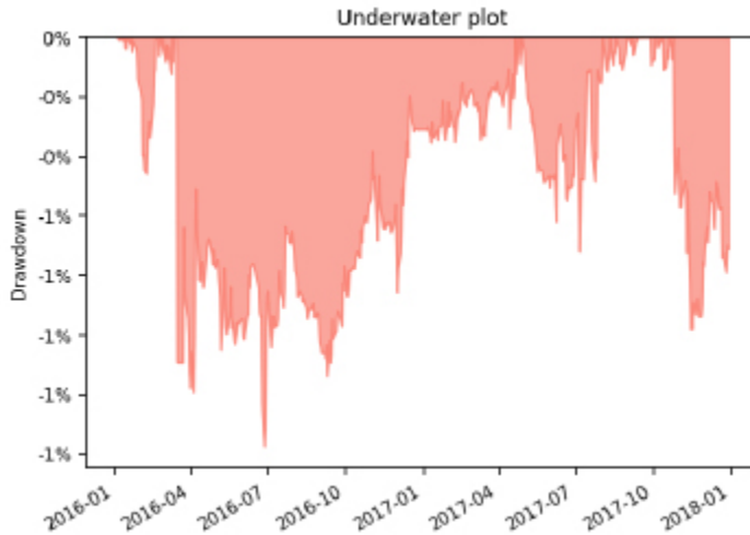
Figure 9.17: Underwater plot visualizing the strategy drawdown amounts
