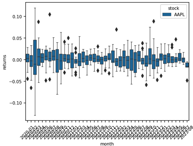
Figure 3.10: Box plot showing monthly summary statistics for AAPL returns.
